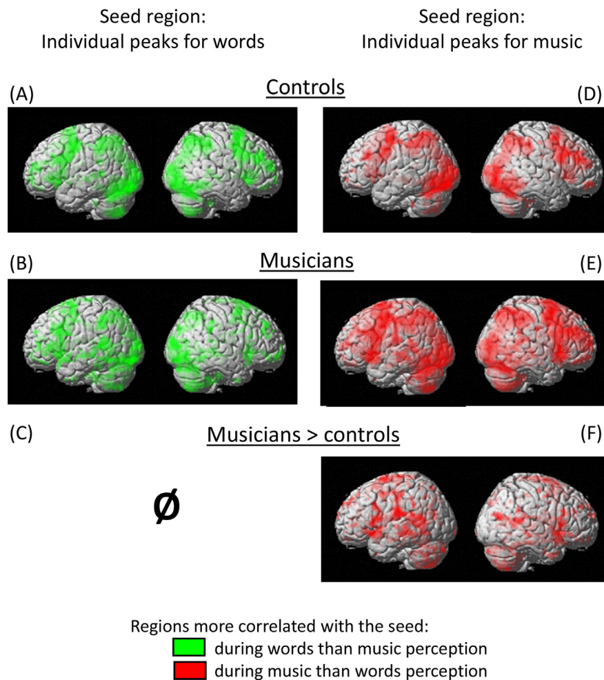
Fig. 6 – Functional connectivity of ventral visual cortex during the processing of written words and music. Left occipitotemporal word-selective and music-selective ROIs were identified in each subject (see Fig. 4). Psycho-physiological interaction (PPI) analysis assessed which brain regions were correlated with the word ROI (left column) and the music ROI (right column), during word more than music perception (green), and during music more than word perception (red), separately for musicians and controls. A set of left-predominant language-related regions were more connected to the word ROI during word reading than during music viewing in controls (A) and musicians (B), with no difference across groups (C). A bilateral network was more connected to the music ROI during music than during words viewing in controls (D) and musicians (E), with a strong predominance in the latter group (F).
