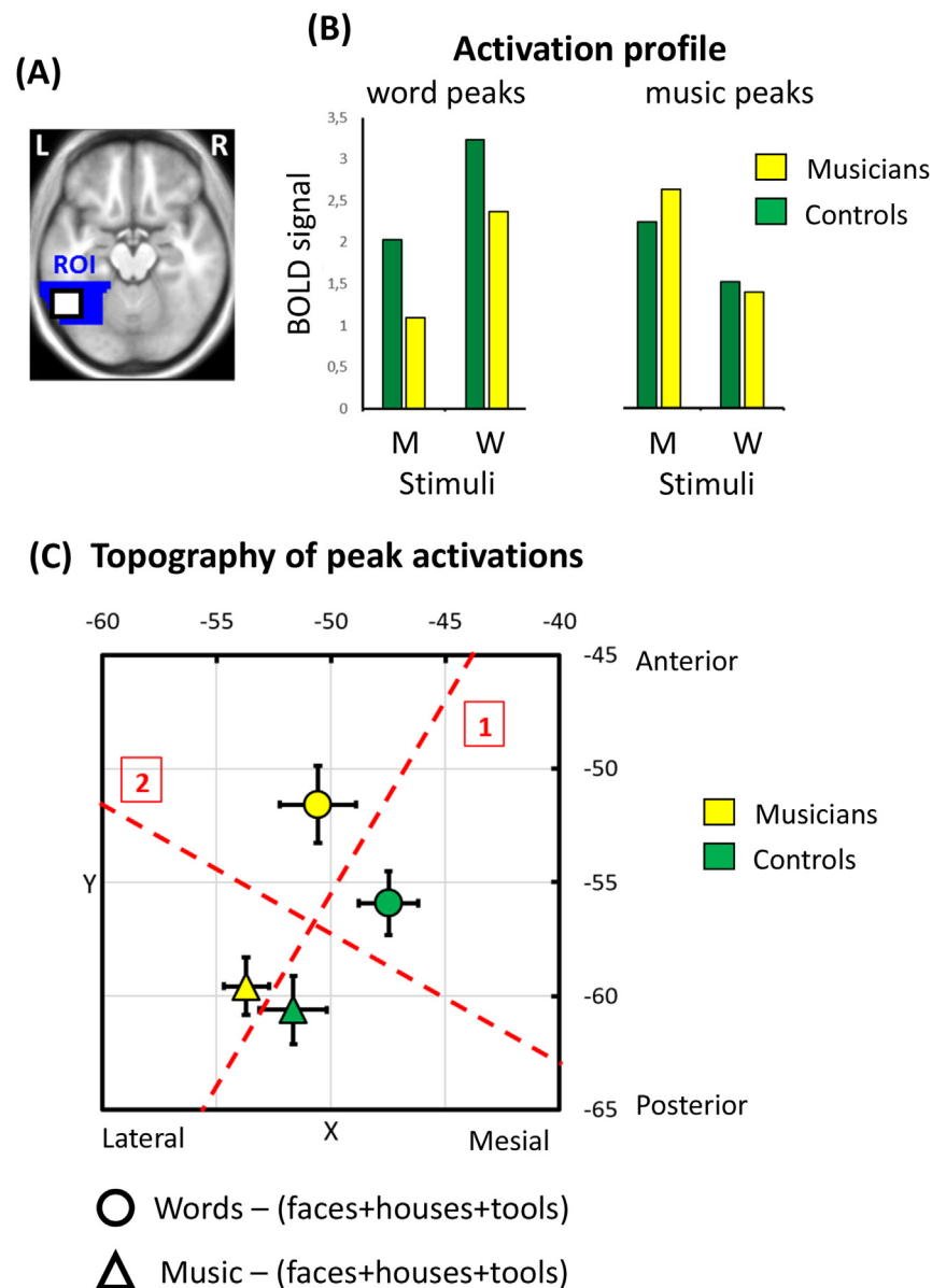
Fig. 4 – Analyses of individual left occipitotemporal activations to music and words. (A) Individual peaks were identified within a left occipitotemporal region of interest (blue). (B) Mean amplitude of activations at individual peaks, showing larger activation at word peaks for words (W) than music (M), and larger activation at music peaks for music than words, both in musicians and controls. (C) Mean MNI x and y coordinates ( \pm 1 SEM) are shown for music (triangles) and words (circles), in controls (green) and musicians (yellow). The first two axes of the PCA are shown in red. Activations for music were posterior and lateral to activations for words, and activations for words were more anterolateral in musicians than in controls.
