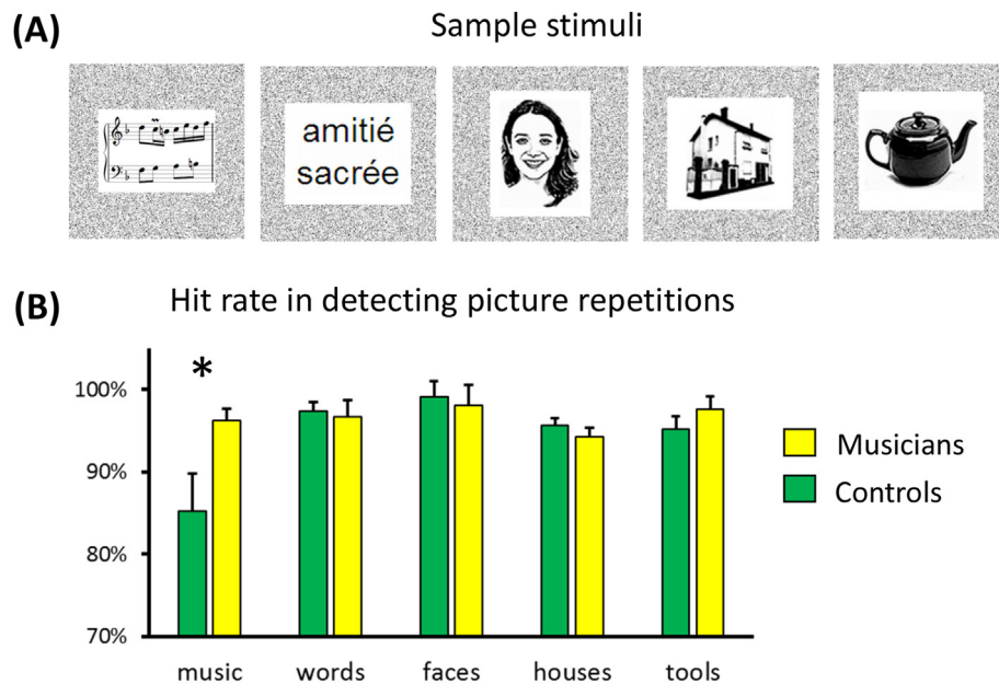
Fig. 1 – (A) Examples of stimuli used in the fMRI experiment. (B) Hit rate in detecting repetitions of words, faces, houses, tools and music scores, in musicians (yellow bars) and controls (green bars). Musicians were more proficient than controls with music scores ( p = .025 ).
